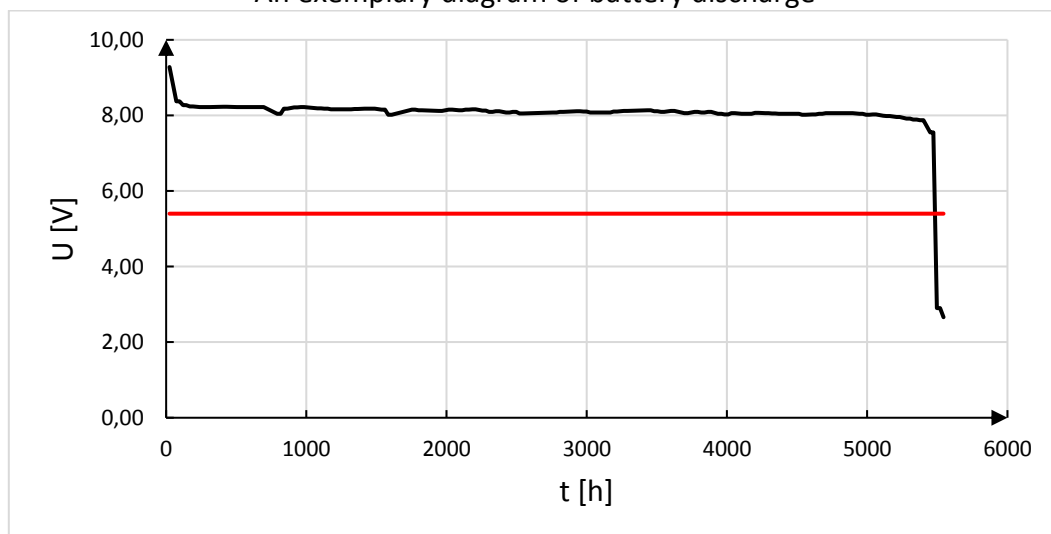
An exemplary diagram of battery discharge
